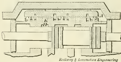
Fig. 3.—WIDE OPEN.
